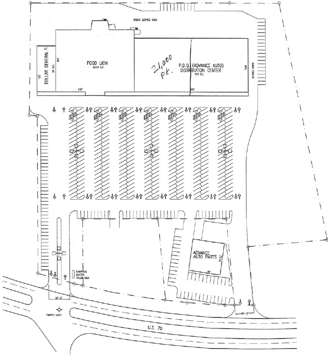
A SITE PLAN SCALE: 1" = 50'
